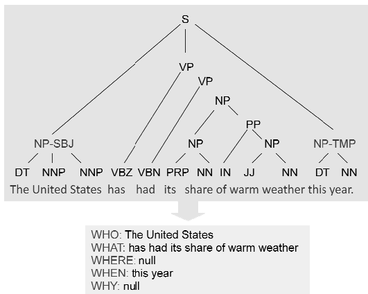
Figure 2: The function tags assist in finding the subject, object, and arguments of a given predicate.
